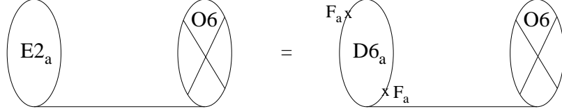
Figure 1: Relation between instantonic one-loop amplitudes and corresponding gauge threshold corrections
