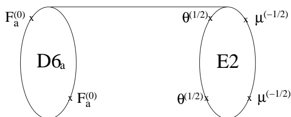
Figure 3: Deformations of an instanton which is invariant under the orientifold projection
