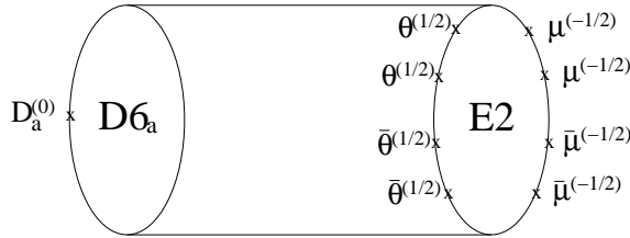
Figure 5: Annulus diagram for E2-instanton correction to \xi_a . The upper indices give the ghost number of the vertex operators.
